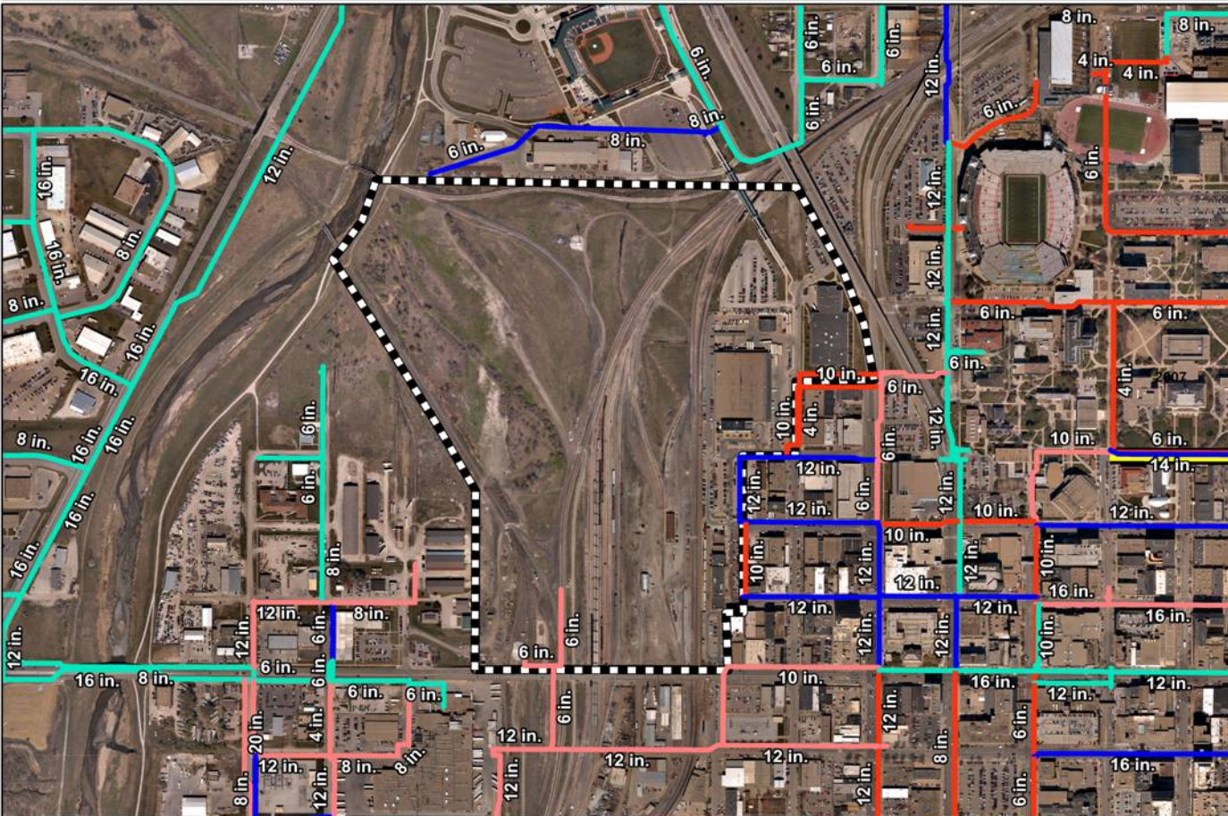
Age and Size of Lincoln Water Mains in West Haymarket Area Study Area Boundary Arena/Expo Center Task Force
