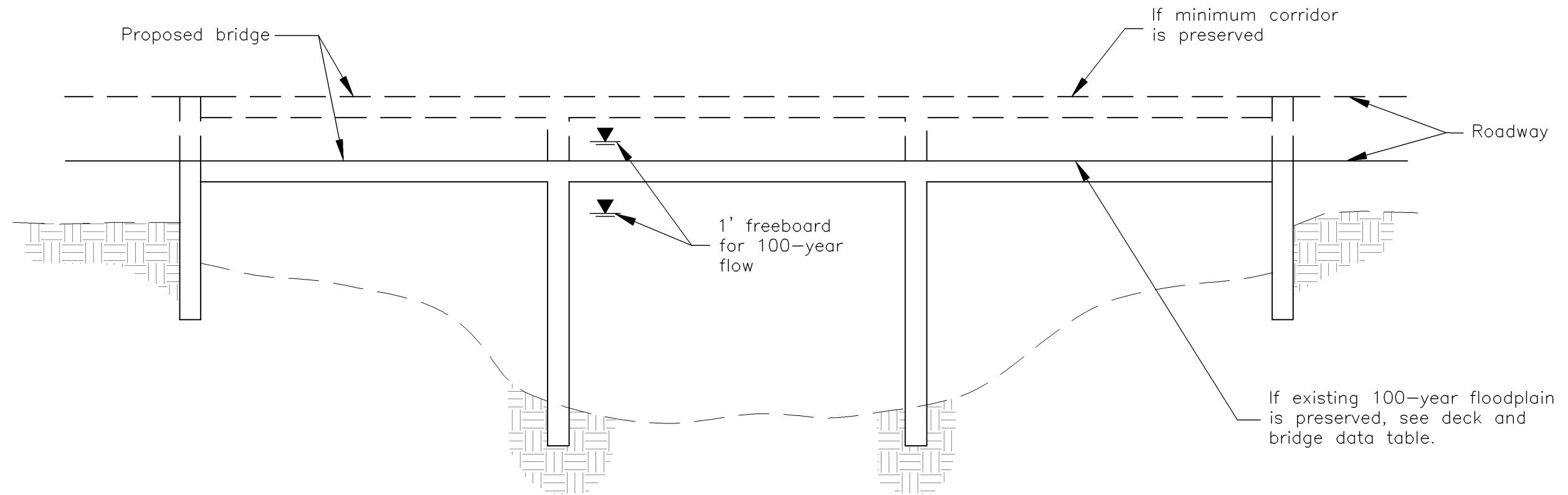
TYPICAL BRIDGE CROSSING N.T.S.
