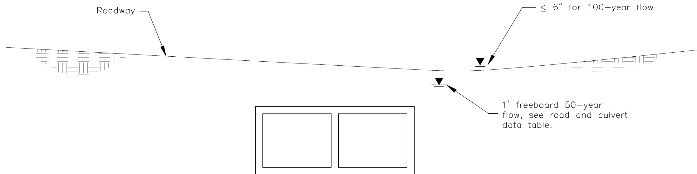
TYPICAL CULVERT CROSSING N.T.S.
