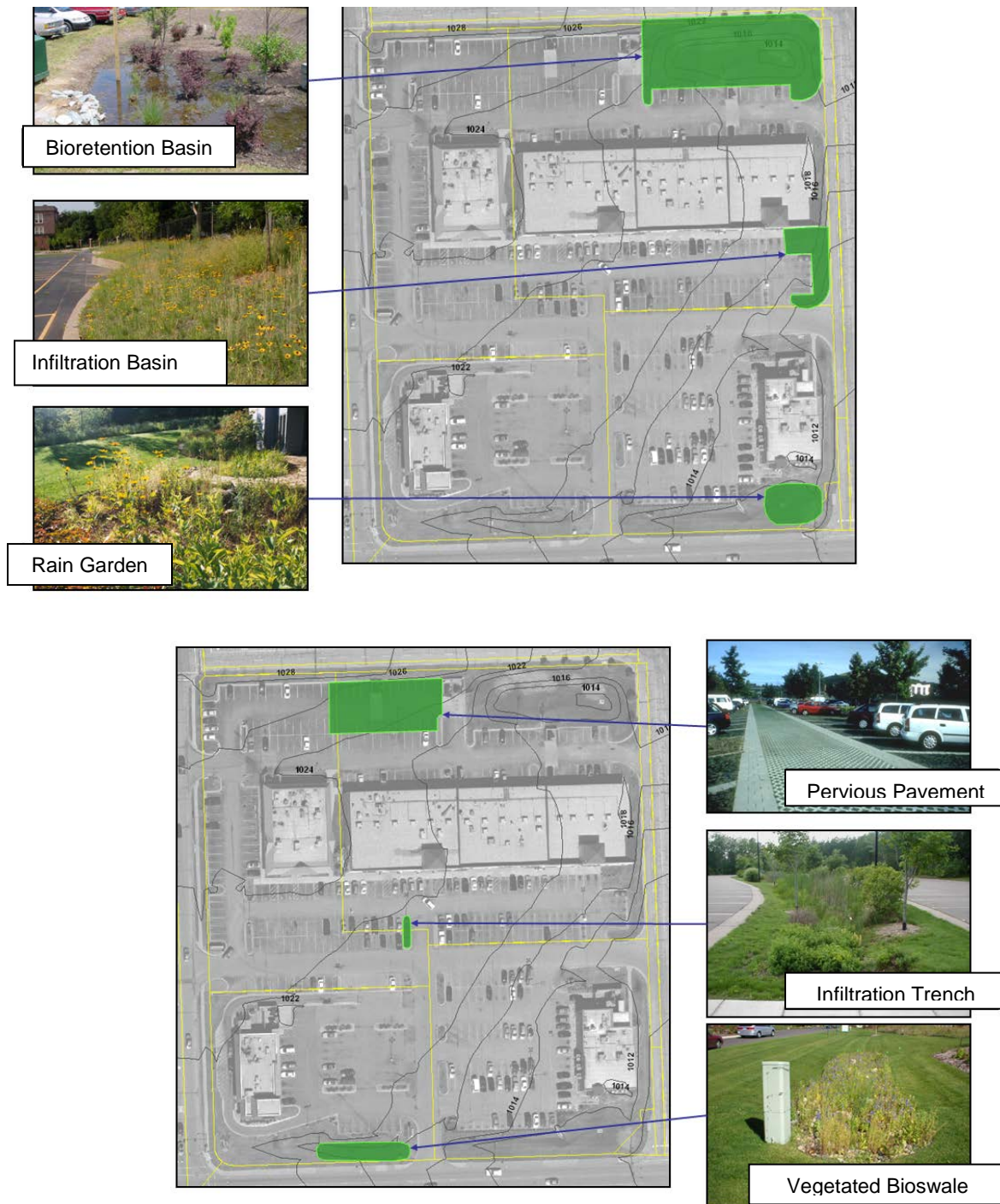
Figure 2: Examples of potential BMP applications in a commercial parking lot
