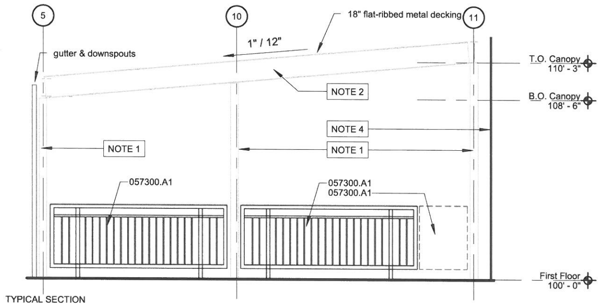
TYPICAL SECTION
