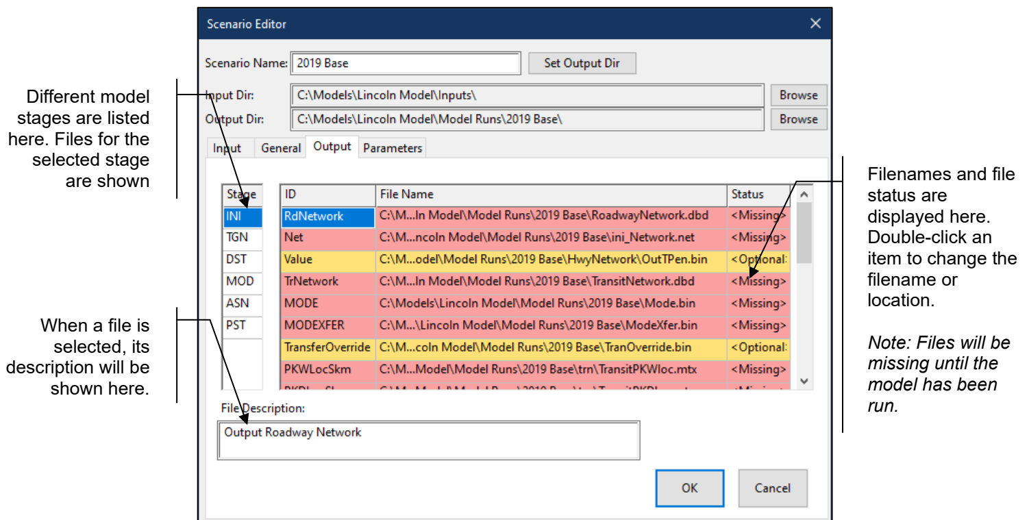
Figure 3.4 The Scenario Editor (Output Tab)
