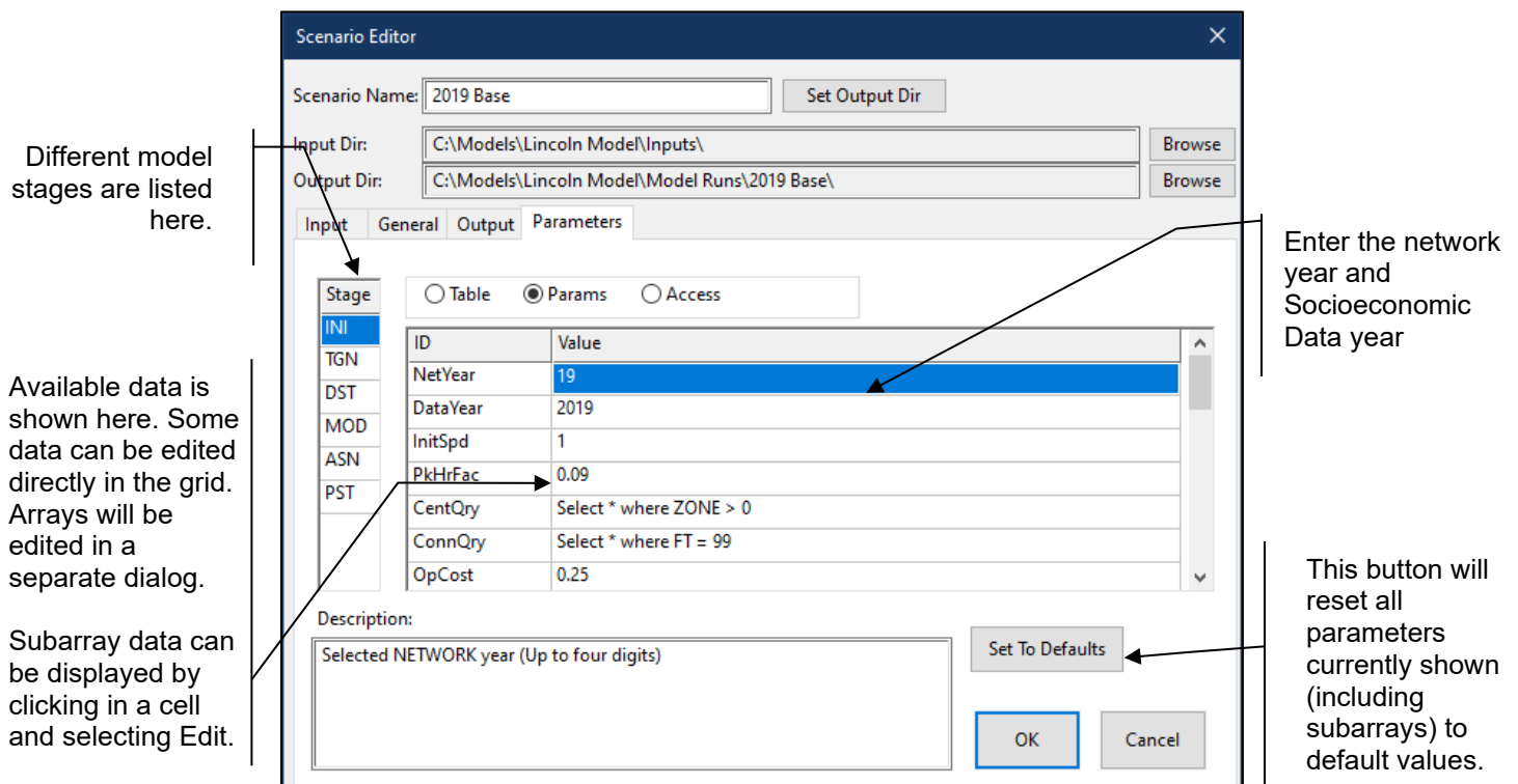
Figure 3.5 The Scenario Editor (Parameters Tab)
