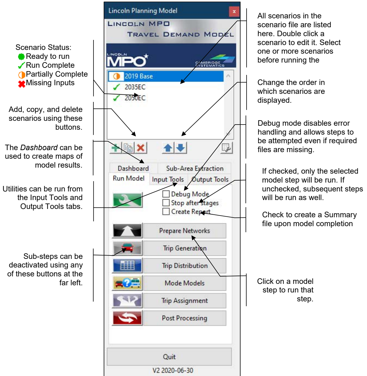
Figure 3.1 The Model Dialog Box (Scenario Management)
