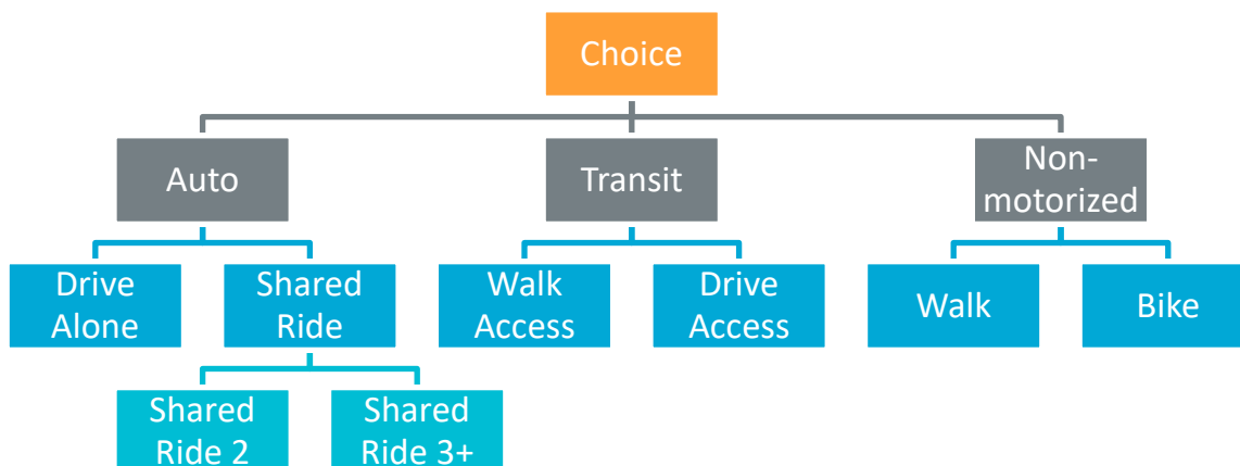
Figure 5.1 Nested Logit Mode Choice Structure
