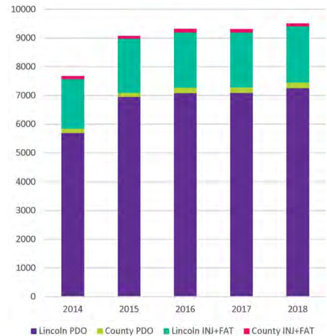
Figure 4.51 Crash Severity
