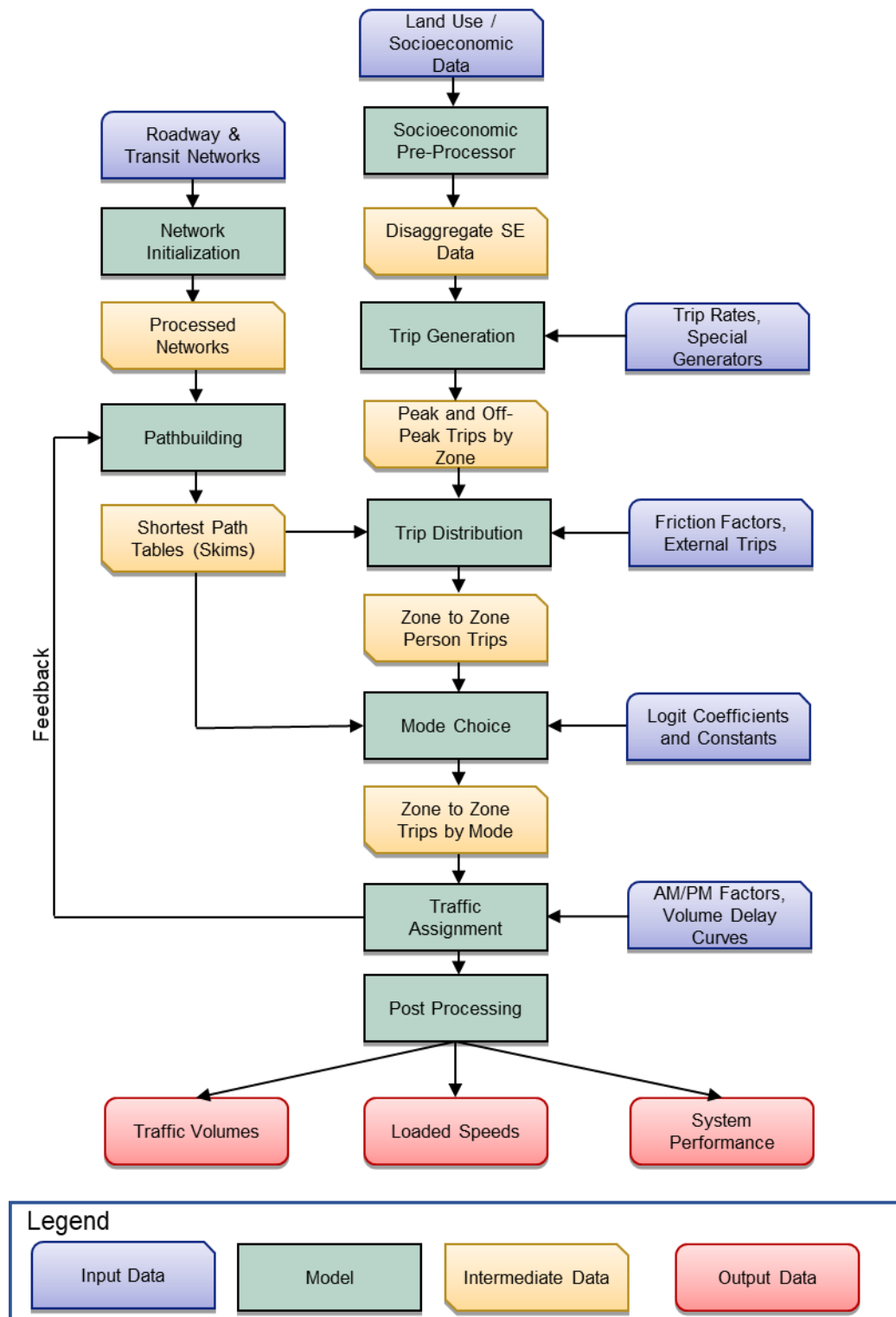
Figure 1.1 Model Flow Chart
