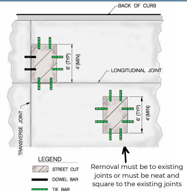
Reinforcement Detail
