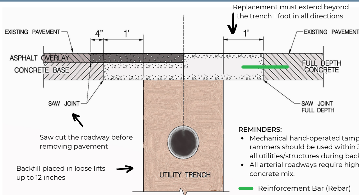
Street Cut Detail
